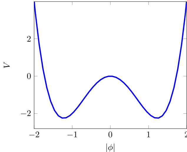
Figure 7: Scalar field potential
