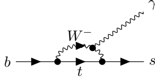
Figure 8: b \rightarrow s\gamma
